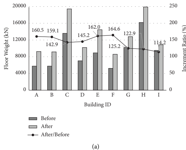
FIGURE 8: Variation of the floor weight and unit floor weight after remodeling: (a) floor weight and (b) unit floor weight.
