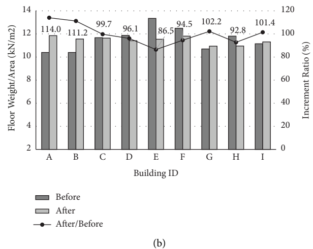
FIGURE 8: Variation of the floor weight and unit floor weight after remodeling: (a) floor weight and (b) unit floor weight.
