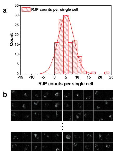
Figure 5. Verification of quantitative RJP phagocytic properties of RAW264.7 cells to (a) distribution of cell counts versus phagocytosed RJP counts in the cell body. (b) Microscopic retroreflection images of single cells having engulfed various numbers of RJPs. (Each grid is 55 \times 55 \mu\text{m}^2 in size).
