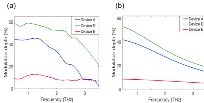
Fig. 4. Modulation depth of device A (blue), device D (green) and device E (red) with respect to frequency, obtained (a) experimentally, and (b) by calculation.
